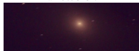
Andromeda Galaxy: M31 was a 30sec exposure at ISO200, using Don's Orion 8" Newtonian Astrograph taken and taken by Terry Dancer
